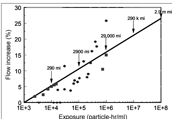
Figure 2: Fuel injector nozzle wear represented by increase in fuel flow as a function of particle concentration. Assumption 2 ppm fuel.
