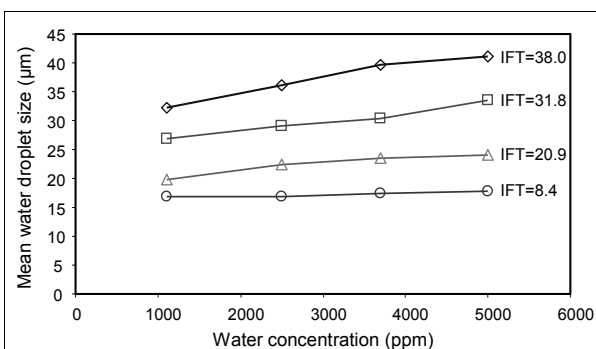
Figure 4: Mean droplet size as a function water concentration and IFT.
