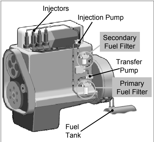
Figure 11: A typical fuel systems with both primary and secondary fuel filters.
