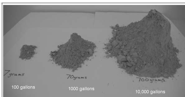
Figure 15: Amount of ISO medium laboratory test dust required to contaminate fuel to an ISO cleanliness of 22/21/18, or alternatively which must be filtered out of the given fuel volume.
