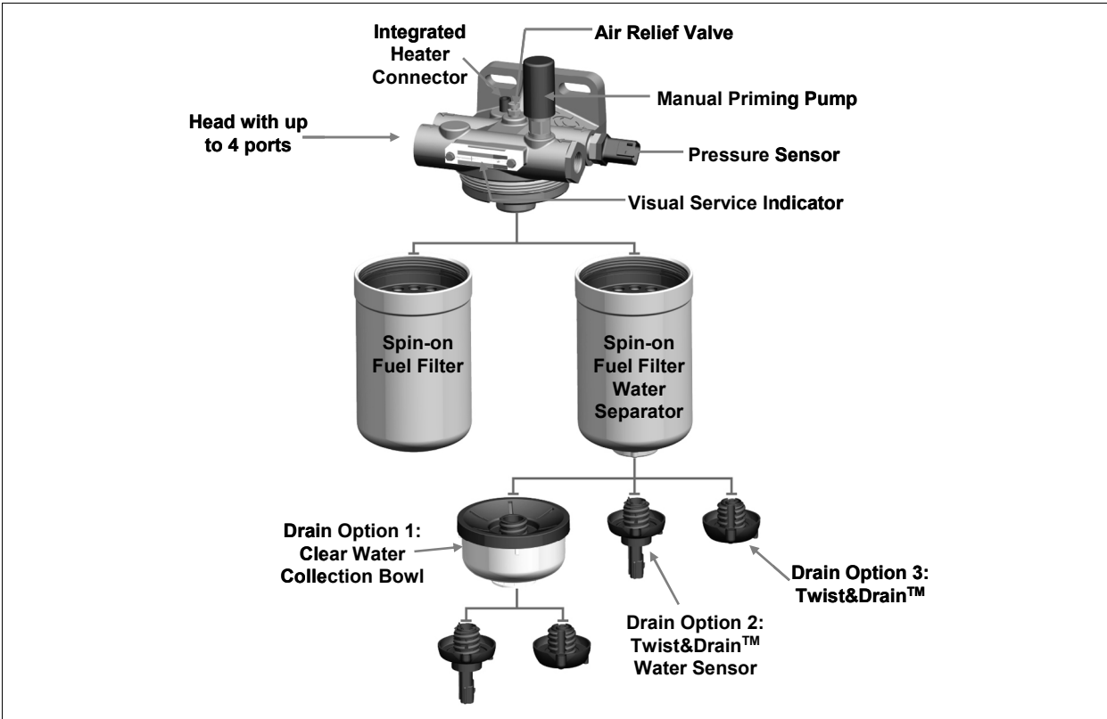
Figure 10: Remote mount fuel filtration assembly with optional features and functions.
