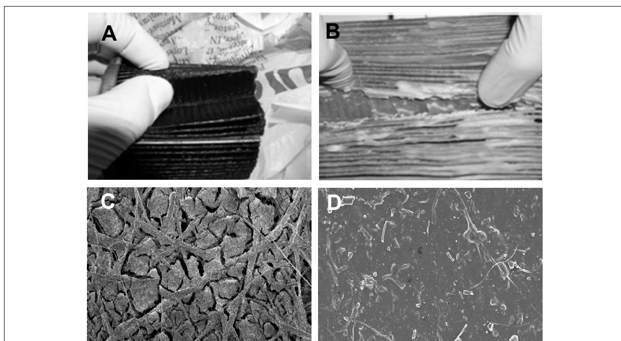
Figure 5: A) plugged ULSD fuel filter, B) plugged biodiesel fuel filter, C) SEM of ULSD formed organic contaminants, and D) SEM of biodiesel formed organic contaminants.
