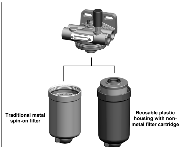
Figure 9: Example of metal spin-on ( left ) and replaceable filter element cartridge ( right ).
